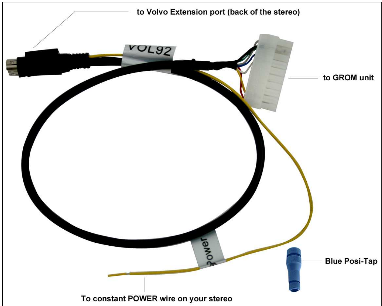
Picture 1: VOL92 vehicle specific harness and Posi-Tap
