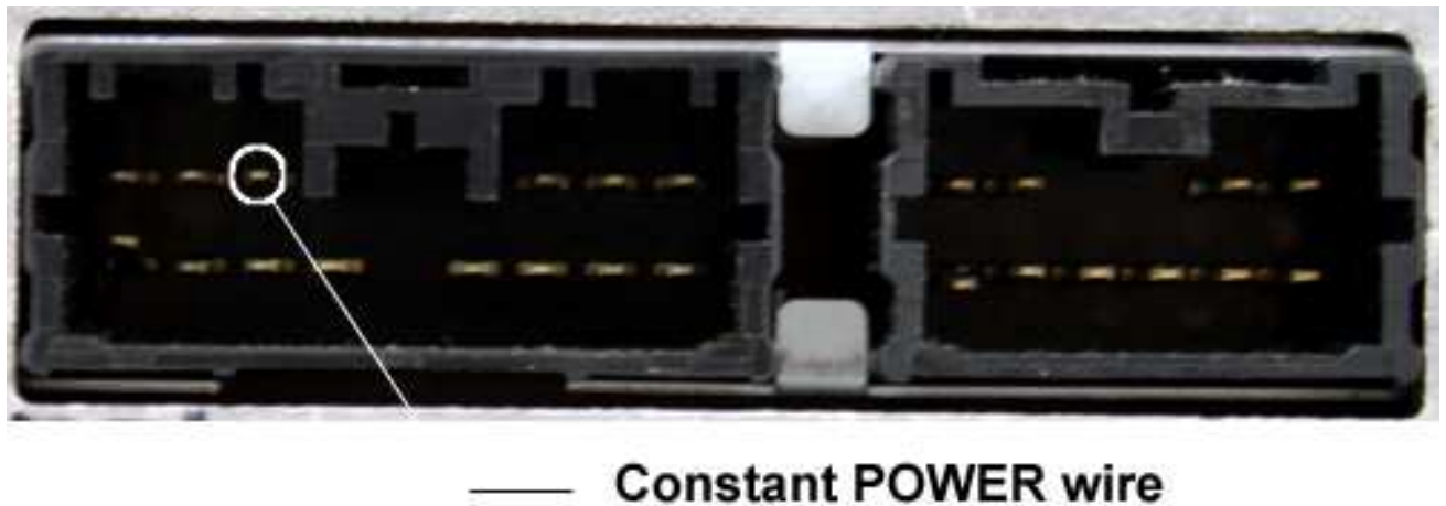
Picture 3: Constant POWER wire location on the main vehicle harness
