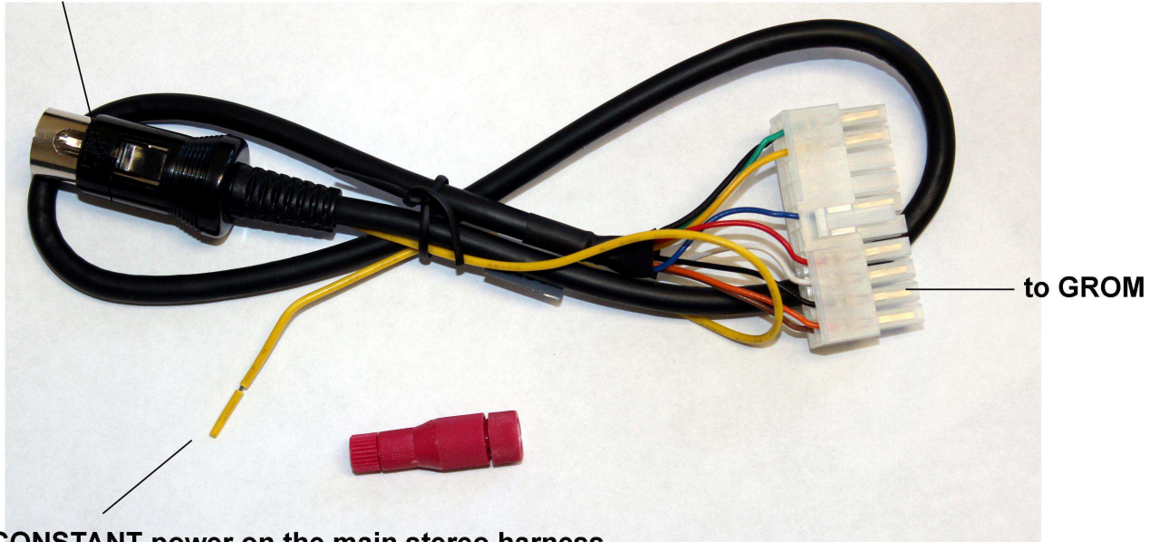
Picture 1: MITS02 vehicle specific harness
